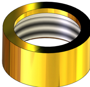
5/8" Cap .610 diameter 9/16-28 thread
