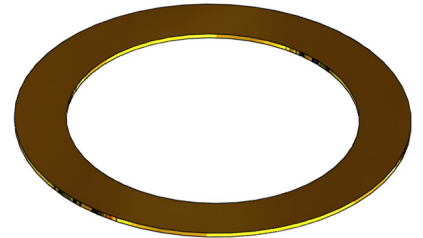
Friction Ring For 1-1/2" Closet Spud CS150-B 2.625" x 1.940" x 0.031"
