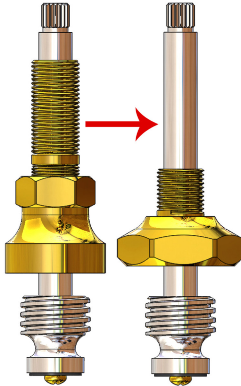
S/V Unit 412101 4.84" With original bonnet
