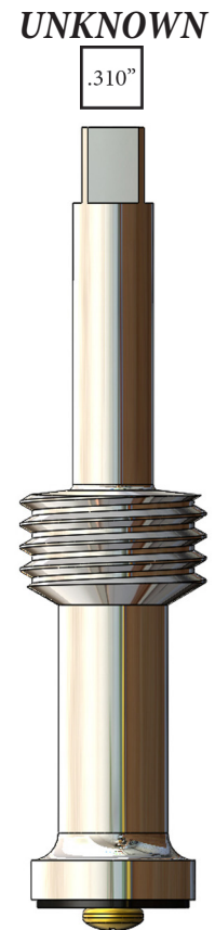
S/V Stem 204381 3.83"
