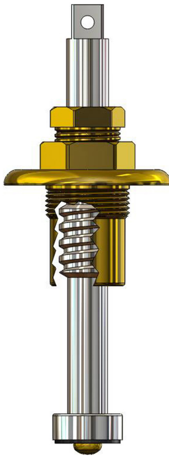
Stem Unit 407701 4.680"
