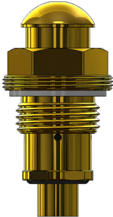
Drinking Fountain Push Button Unit
