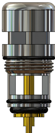
Push Diverter 431720 2.40"
