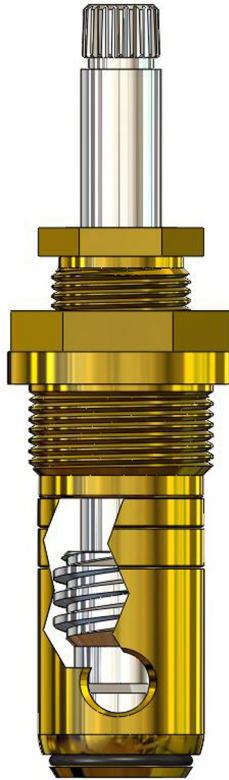
Stem Unit LF472061 LF472062 4.060"
