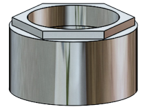
O.D.: 1.10" HEIGHT: .630" OEM: RP5861 CHROME CAP NUT
