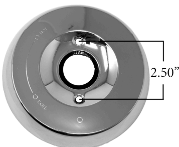
KO50433 FOR KOHLER
