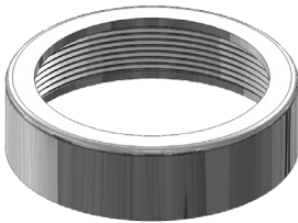
O.D.: 2-1/8" HEIGHT: .590" THREAD: 2"-20 OEM#: RP22734 NICKEL PLATED BONNET NUT
