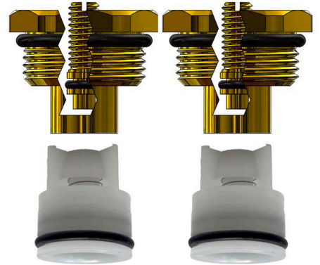
Check Stop Unit 400011-KIT OEM: 130158
