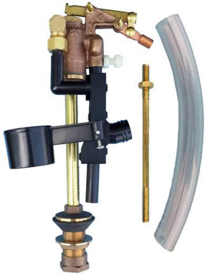
Scovill Model 16AK Anit-Siphon Ballcock for Kohler*
