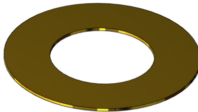
Friction Ring For 1" Urinal Spud CS100X075-B 1.935" x 1.030" x 0.031"
