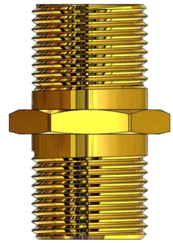
Ballcock Nipple Male 15/16-14 X 2-1/8" Hex 1.88" Long
