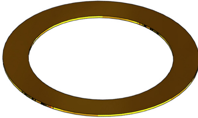
Friction Ring For 1-1/2" Closet Spud CS150-B 2.625" x 1.940" x 0.031"
