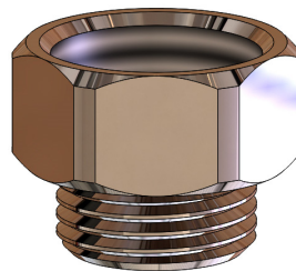
Ballcock Shank Adapter Male 1/2-14 NPS X Female 15/16-14
