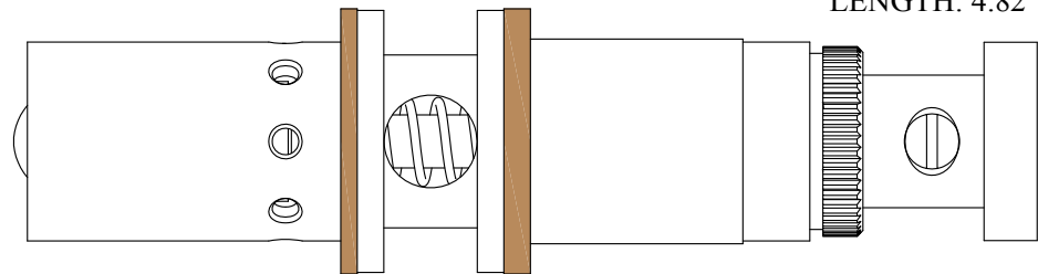
475700 GASKET: 894650 INCLUDED FOR PILOT Flush Valve
