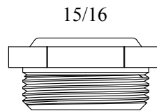
649530 AM. STD.*
