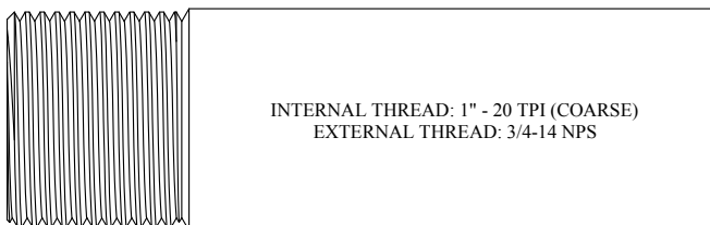
SLEEVE
