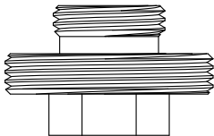
1-7/32-18 x 3/8-18 NPS 125340
