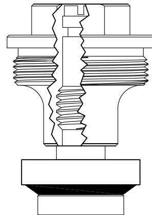
460401 FOR SPEAKMAN Stop Unit Assembly
