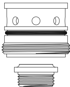
106090-OS SYMMONS TA-4* OLD STYLE (SHORT)
