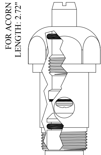
LF401781 OEM# 2767-010-002 LF254071 Stem Only
