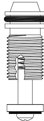
STOP UNIT FOR SENTINEL VALVE
