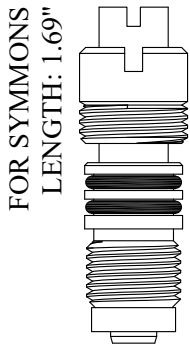
400661 200661 Stem Only OEM # T-52 OEM # T-52A or NS-18
