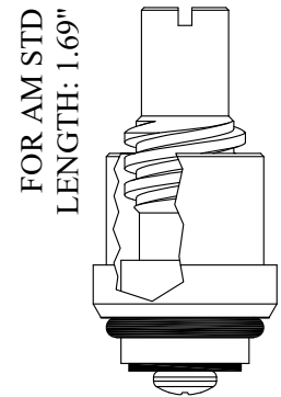
GASKET: 891130 O-RING INCLUDED 453181 253181 Stem Only OEM # 1011-14
