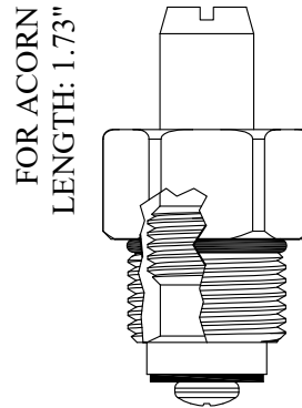
GASKET: 890160 O-RING INCLUDED LF454071 LF254071 Stem Only OEM # 2755-000-002 OEM # 2755-000-001
