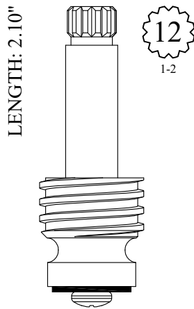
LF259251
