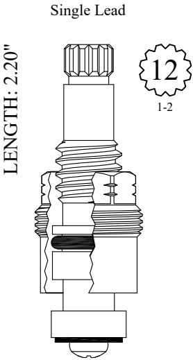
LF461231 OEM # 910-412
