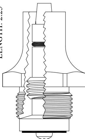
483121 OEM # 0485-000-002
