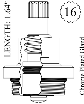
LF453141 OEM # 61509-04
