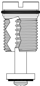
LF400190 OEM # 2415-000-001
