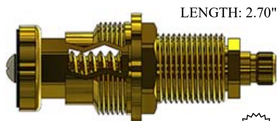
402022 GASKET INCLUDED: 895350
