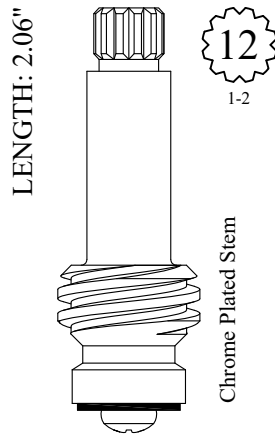
LF260081 LF260082
