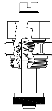
400151 OEM # RP2090
