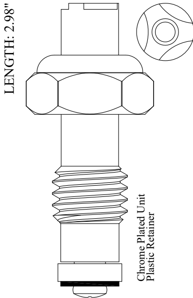
401731 201731 Stem Only OEM # S21-020
