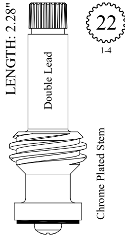
LF263231 OEM # 31286-04 LF263232
