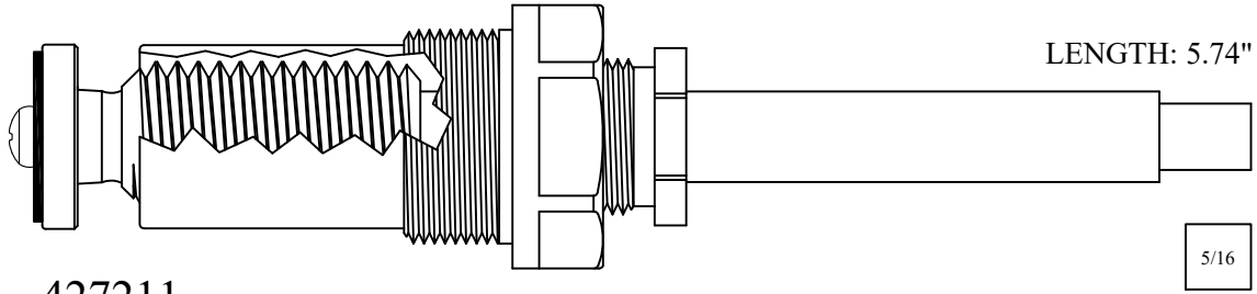
427211 GASKET INCLUDED: 895540 227211 Stem Only
