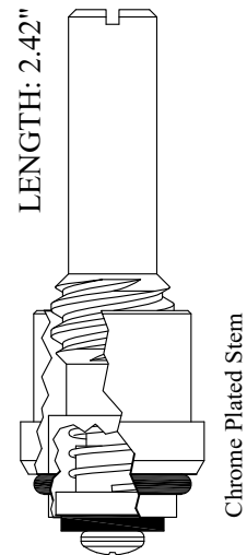
464221 OEM # 521-34 264221 Stem Only OEM # 25317-04
