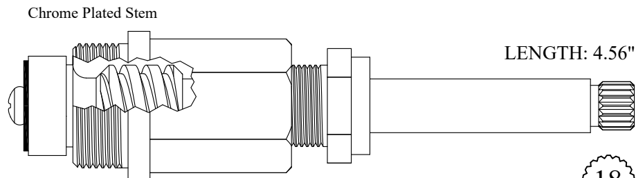
407501/ 407502 GASKET INCLUDED: 895370 207501/ 207502 Stem Only
