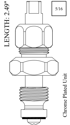
LF463851 LF263851 Stem Only
