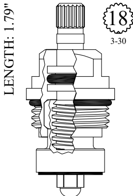
GASKET: 890180 O-RING INCLUDED LF455362
