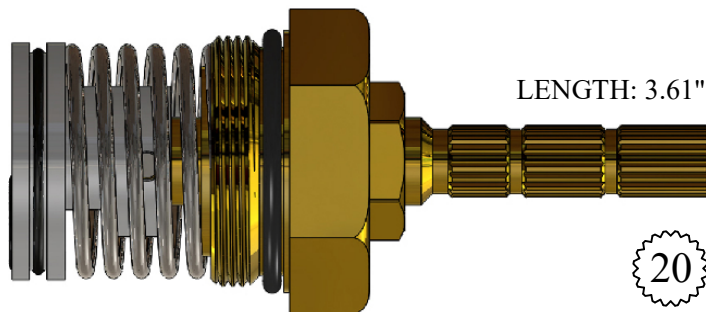
431770 GASKET: 891220 O-RING INCLUDED
