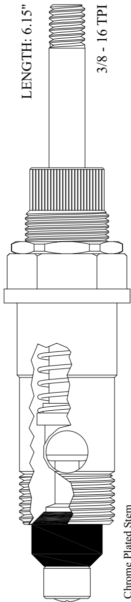
438200 GASKET INCLUDED: 895440 238200 Stem Only
