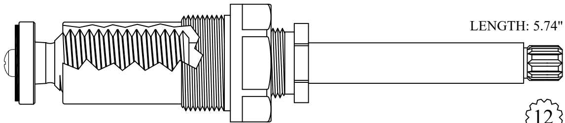
427261 GASKET INCLUDED: 895540 227261 Stem Only
