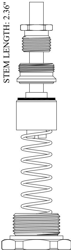
LF152150 Stem Only LF124660 Repair Kit OEM # 66298-0070A
