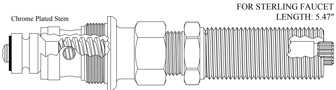
434011 234001 Stem Only GASKET: 895560
