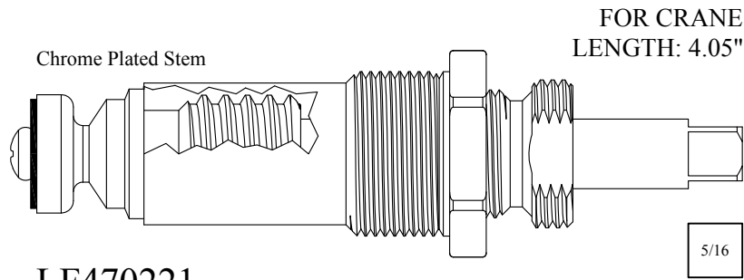
SEAT USED: LF648960
