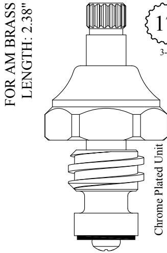
LF464211 LF464212 LF264211 Stem Only LF264212 Stem Only
