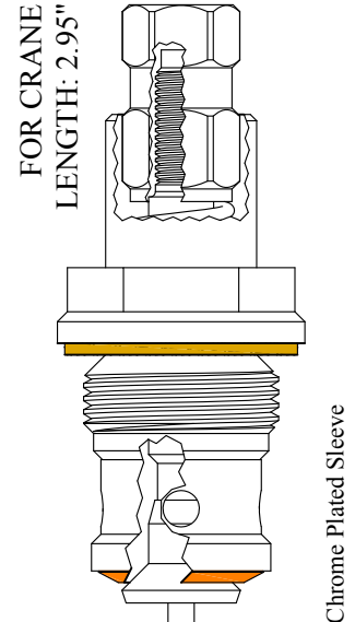
LF465150 LF265150 Stem Only
