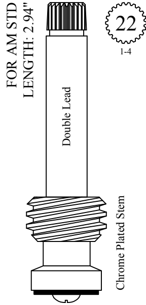
LF266151 LF266152 USES BARREL: LF647041/LF647042
