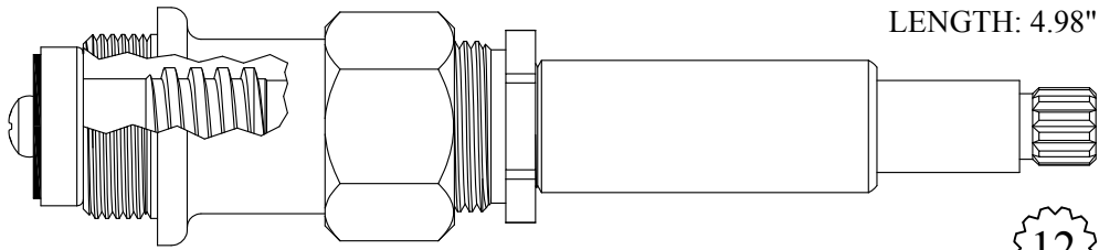
Chrome Plated Stem & Esc Tube
