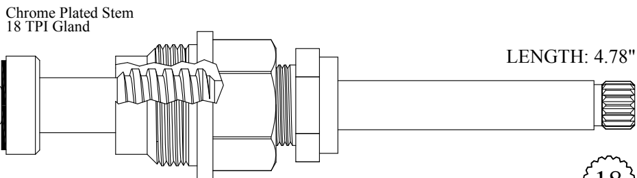
Chrome Plated Stem 18 TPI Gland 409701 209701 Stem Only GASKET: 895370
