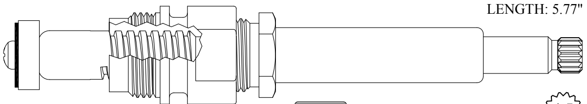
Chrome Plated Stem & Esc Tube
