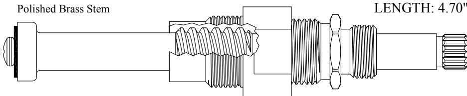
Polished Brass Stem
