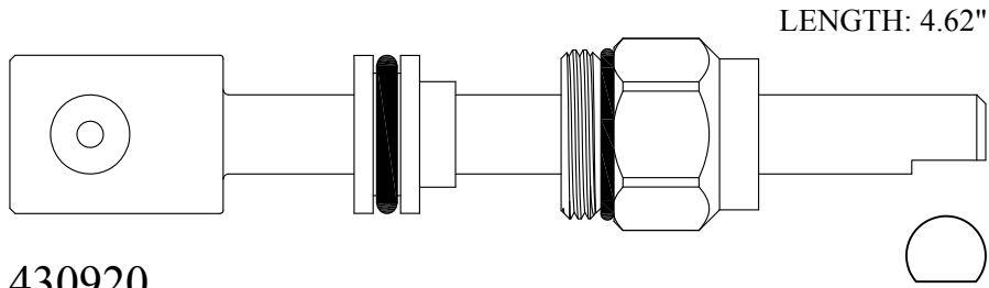
430920 230920 Stem Only GASKET: 890170 O-RING INCLUDED
