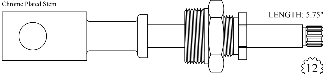
436270 236270 Stem Only GASKET: 895550
