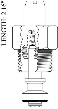
LF400571 LF200571 Stem Only
