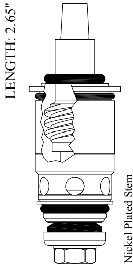
NEW STYLE QUATURN
