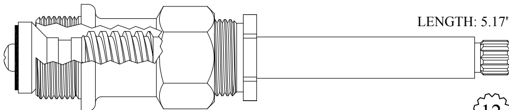
Chrome Plated Stem
