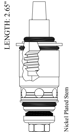
NEW STYLE SLOW COMPRESSION
