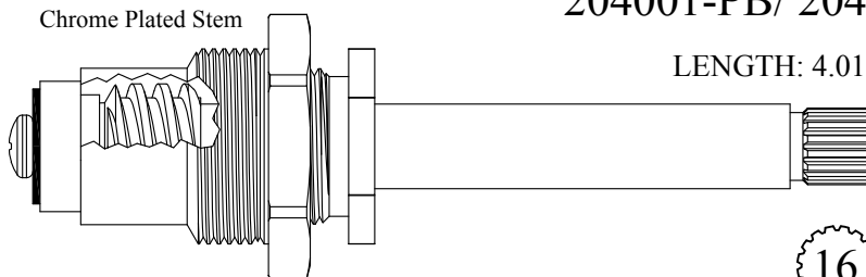
SEAT USED: LF649640
