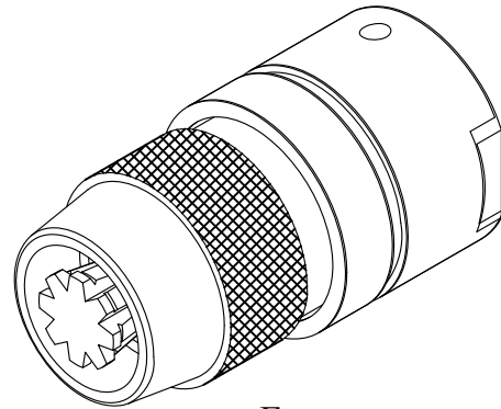
For Symmons "Free-Flo" Rigid OEM# 4-285F 112620: 2.5 GPM
