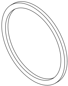
1.562 x 1.375 x .062 GASKET
