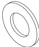
.860 x .468 x .050 BRASS WASHER
