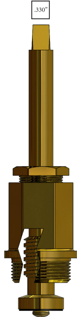
S/V Stem 418461 5.08"
