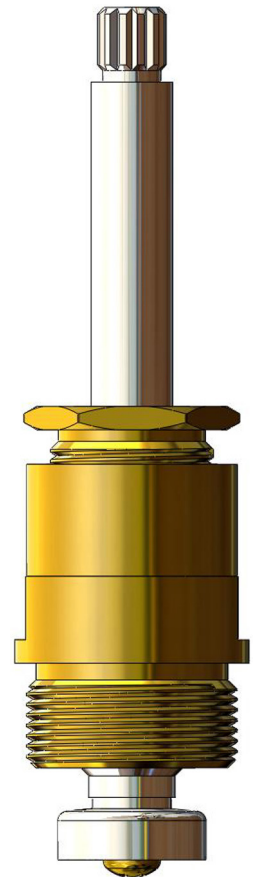
Stem Unit 410041 4.560" 1-1/8" Cap Thread Gasket: 894620
