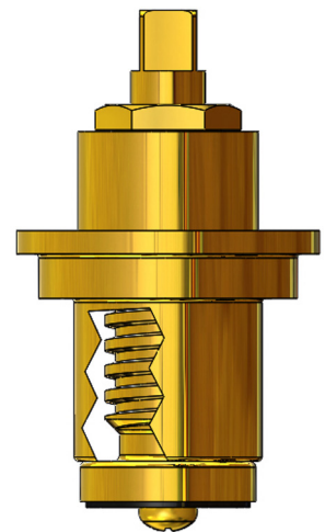
Steam Valve Stem 483511 2.43"
