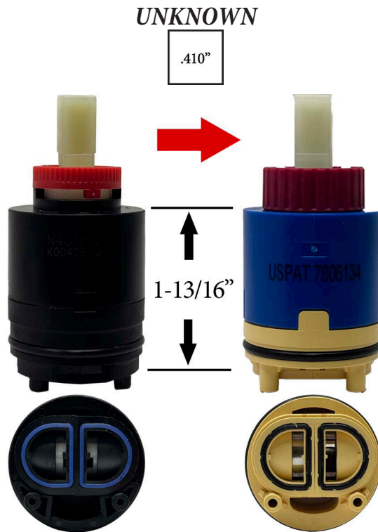
40mm Pressure Balance Ceramic Cartridge
