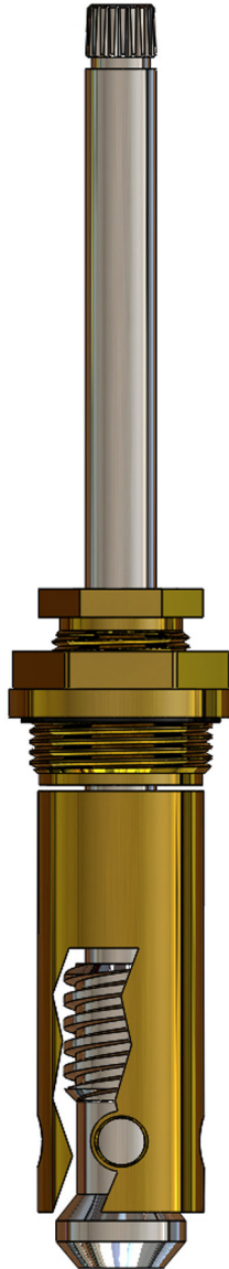
Diverter Unit
