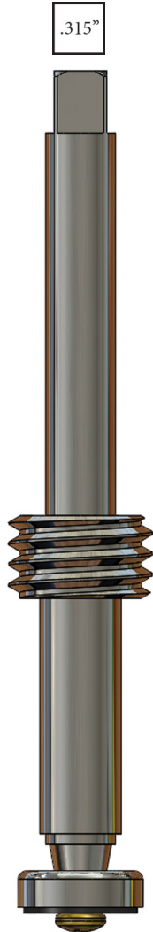
S/V Stem 209181 5.05"
