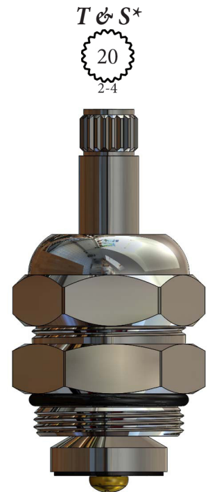
Stem Big Flo Unit LF465781 LF465782 2.88" OEM: 006482-40
