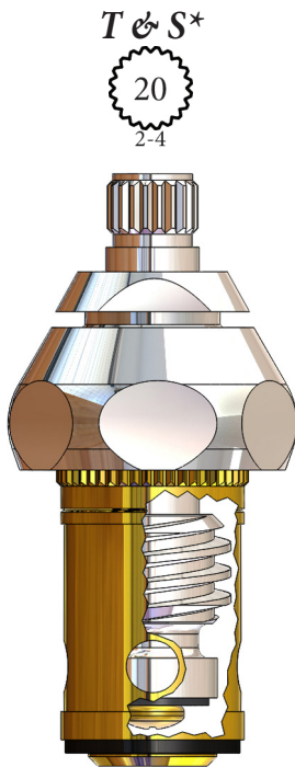
Stem Unit LF464061-NS LF464062-NS 2.83" New Style
