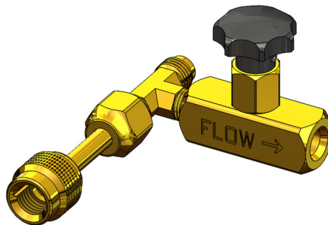
Bleed-Off Valve Assembly 136030 For backflow testing
