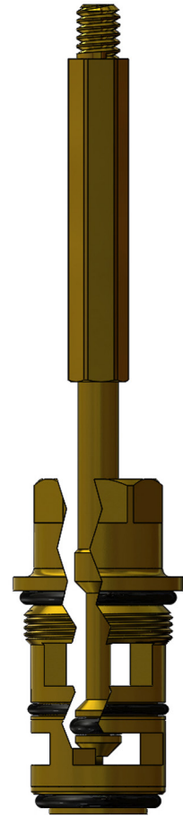
Diverter Unit 432850 4.71"
