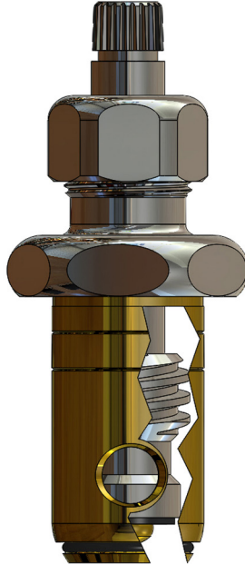
Exposed Stem Unit LF466171 LF466172 3.20"
