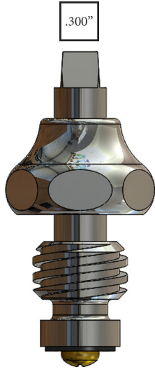
Stem Unit LF461881 LF461882 2.25"
