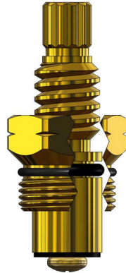
Stem Unit 400801 400802 1.905"
