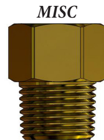
1/2" NPS Female to 1/2" NPT Male Adapter LF151400 1.250" Lead Free
