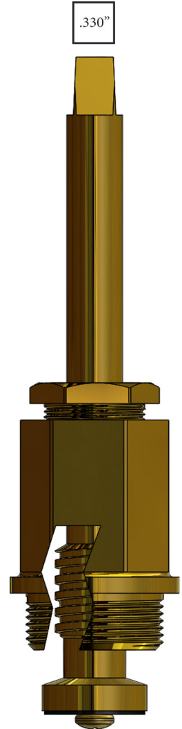
S/V Stem 418461 5.08"
