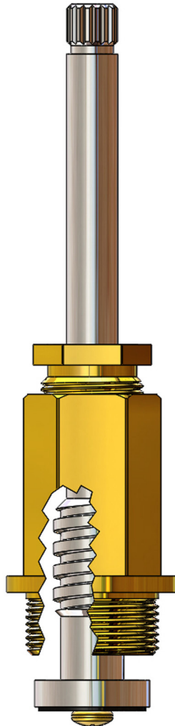
S/V Unit 414001 5.13"
