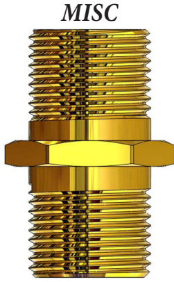
MISC Male 15/16-14 X 2 1/8" Hex Ballcock Nipple 159900 1.88"
