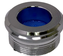
Aerator Adapter LF166170 15/16" Male & 55/64" Female x 3/4-11.5 GHT
