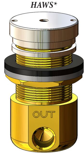
HAWS* Drinking Fountain Valve and Push Button LF163260 3.18" OEM: 5874PB
