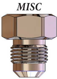
MISC Hose Adapter LF153320 1.035" 3/8" Compression Female X 3/8" Flare Male
