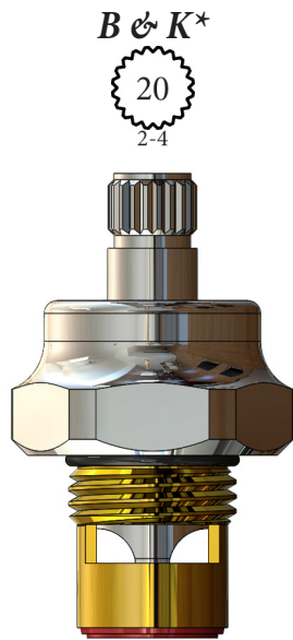
Ceramic Unit LF460311-N LF460312-N 2.20"
