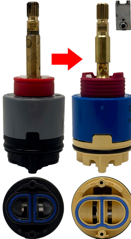
Ceramic Cartridge CC19165 3.97" 40mm O.D.
