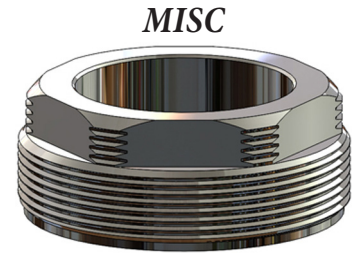
MISC Chrome Plated Nut For Single Handle Cartridge 159830 .690" M43 X 1.25 Cap Thread, M45 X 1.25 Esc Thread For CC19102CHK
