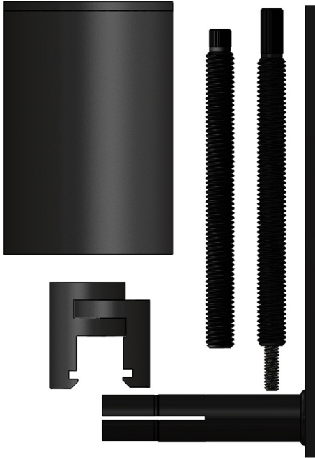
Delta Removal Tools for ONA System
