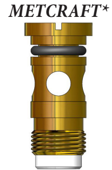
METCRAFT* Flow Cont Assembly LF111950 OEM: 77262, 77344 Part # GPM LF111950 1.0 LF137430 0.7 LF137500 2.5 LF150960 0.5
