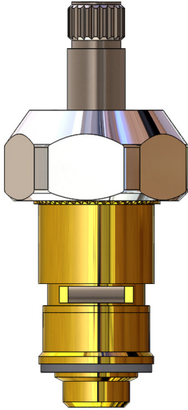
Ceramic Unit LF466401-NS-N LF466402-NS-N 3.045" With New Style Nut OEM: 011278-25NS
