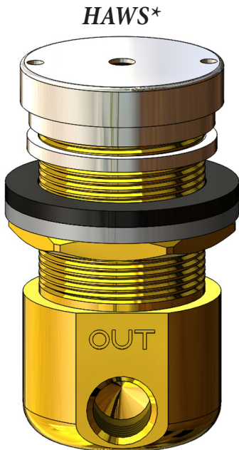
HAWS* Drinking Fountain Valve and Push Button LF163260 3.18" OEM: 5874PB
