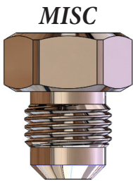
Hose Adapter LF153320 1.035" 3/8" Compression Female X 3/8" Flare Male
