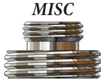
Adapter 154040 .610" 3/8-18 NPS X 3/4-11.5 GHT Adapter
