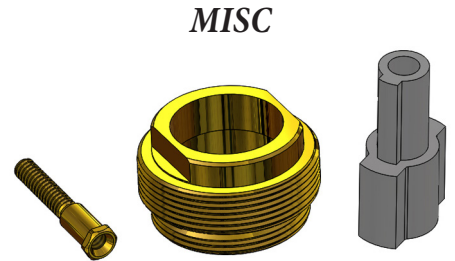
Retrofit Kit for Avante 167600 OEM: 931-930
