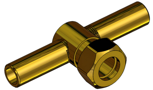
Tee for Prison Lavatory LF160530 OEM: 012498-0070A
