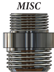
Chrome Plated Adapter LF160990 1.05" 1/2-14 NPS x M18 X 1.25mm
