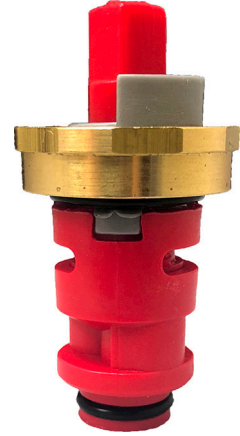
U/R Stem Unit 459621-N 2.250" Includes Bonnet Nut 759620
