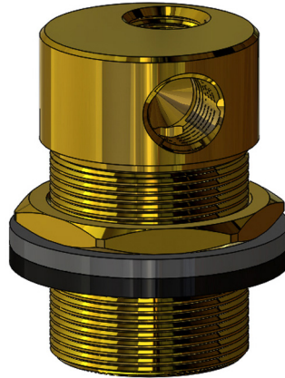
Drinking Fountain Valve Retro Kit LF158470 2.10" Alt design w/out cartridge, Water supply tapped 1/4-18 NPT Includes bubbler nut
