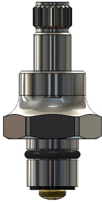
Stem Unit LF462241 LF462242 2.08"
