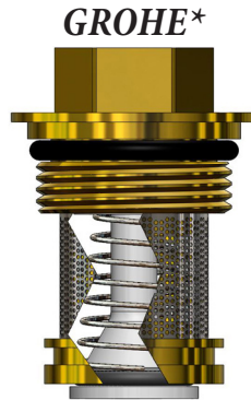
GROHE* Check Valve 142790 1.680" OEM: 08.213
