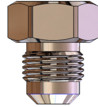
Hose Adapter LF153320 1.035" 3/8" Compression Female X 3/8" Flare Male
