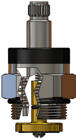
3/4" Compression Cartridge LF465491 LF465492 2.85" OEM: KL34-Y007
