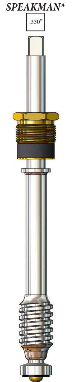
W/S Stem Unit LF480321 7.38"
