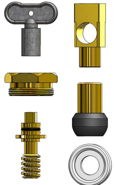
Hydrant Repair Kit 152590 OEM: HK8
