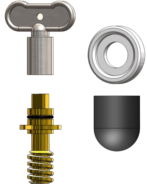
Hydrant Repair Kit 151120 OEM: HK5/#15
