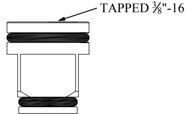
PLUNGER 983060
