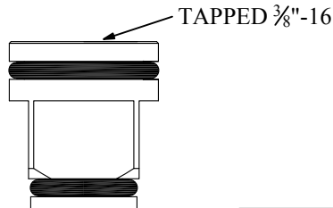
PLUNGER 983060
