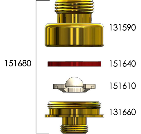
Vacuum Breaker Assembly 151680 Includes 131590, 131660, 151610, and 151640 OEM: WK08
