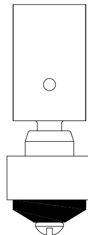
ZURN OPERATING BLOCK & PLUNGER ASSEMBLY (OLD STYLE) 683332
