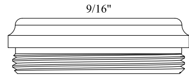
9/16" ZURN HYDRANT SEAT 3/4-16
