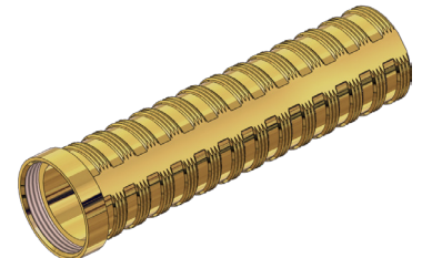
HEIGHT: 3.82" THREADS: M24 x 1.00
