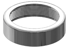
O.D.: 2-1/8" HEIGHT: .590" THREAD: 2"-20 OEM#: RP22734 NICKEL PLATED BONNET NUT
