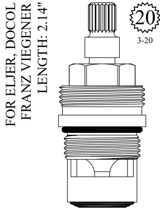
FOR ELJER, DOCOL FRANZ VIEGENER LENGTH: 2.14" GASKET: 890170 O-RING INCLUDED SEAL: 898510 DISC SET: 151380-PKG LF459571 LF459572
