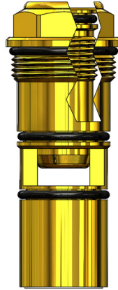
Check Stop Unit - Hot 400540H 2.15" R510 Valve OEM: 953951-0070a
