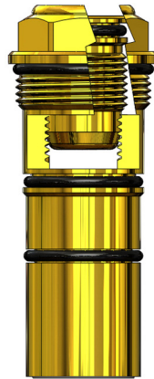
Check Stop Unit - Cold 400540C 2.15" R510 Valve OEM: 953950-0070a
