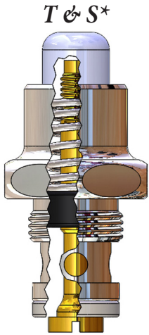
T & S* Knee Valve LF462400-P 2.25" Plastic Button OEM: 002983-40
